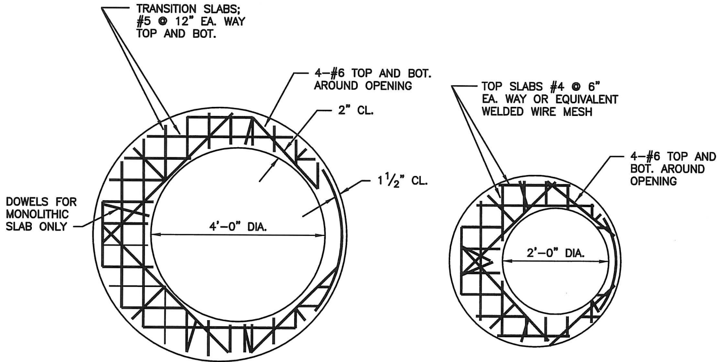
TRANSITION SLAB
